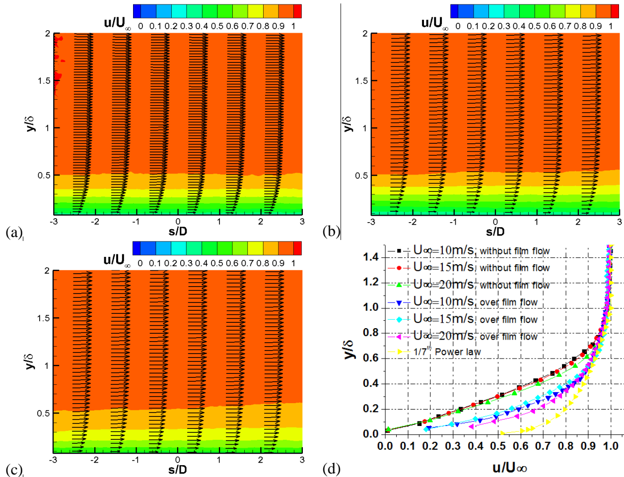
Figure 4-6 Time-average airflow boundary layer over flat plate with film flow. (a) U_\infty = 10\text{m/s} (b) U_\infty = 15\text{m/s} (c) U_\infty = 20\text{m/s} (d) Time-average velocity profiles over flat plate
