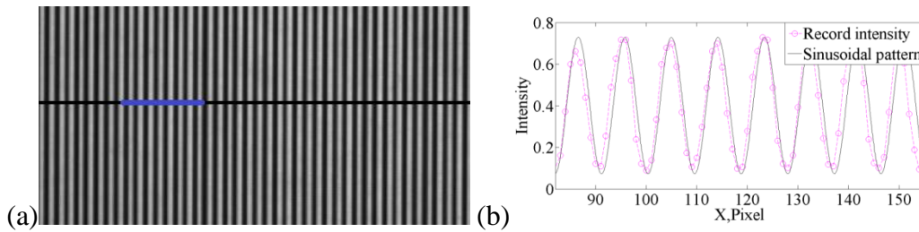
Figure2-7 (a) Projected image pattern. (b) Comparison of normalized image intensity with sinusoidal fitting profile, intensity value from the blue line of left image
