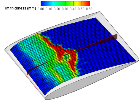
(a). U_\infty = 10\text{m/s} , film front break point
