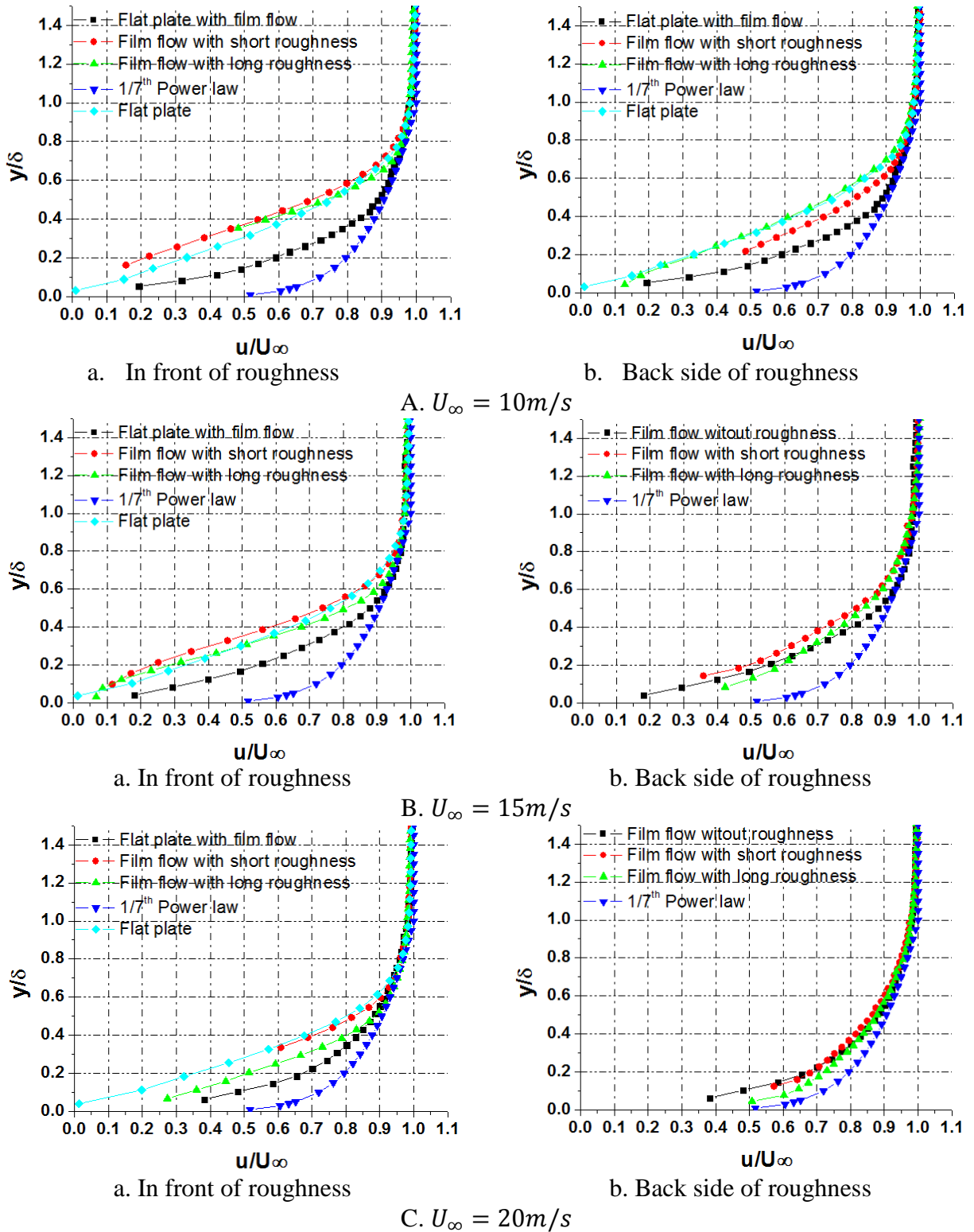
Figure 4-10 Time-average boundary layer velocity profiles in front of and at the back side of roughness for experiment cases with film flow. The location of the velocity profile is s/D = -8 in front of the roughness and s/D = 8 at the back side of roughness
