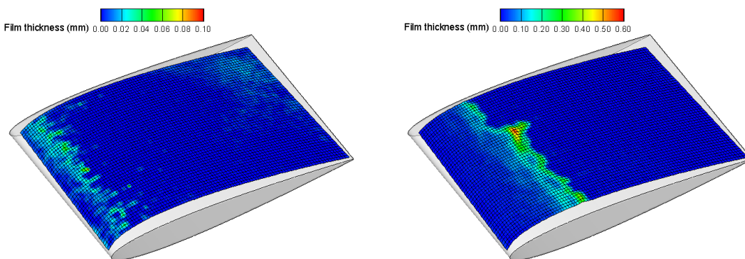
Figure 5-3 DIP measurement results of wind speed U_{\infty}=10m/s .
