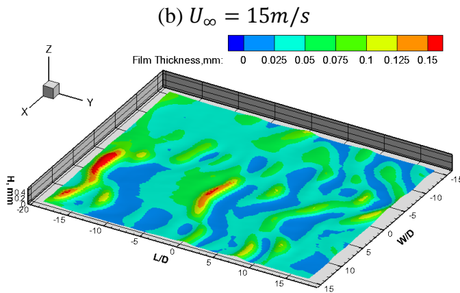
Figure 4-11 Instantaneous film thickness measurement results of the wind-driven water film flow over flat plate at the water flow rate of q=25.3 ml/min/cm
