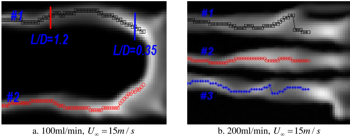
Figure 3-10 Rivulet maximum height location
